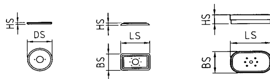
Round Suction Foot Rectangular Suction Foot Sack Suction Foot
